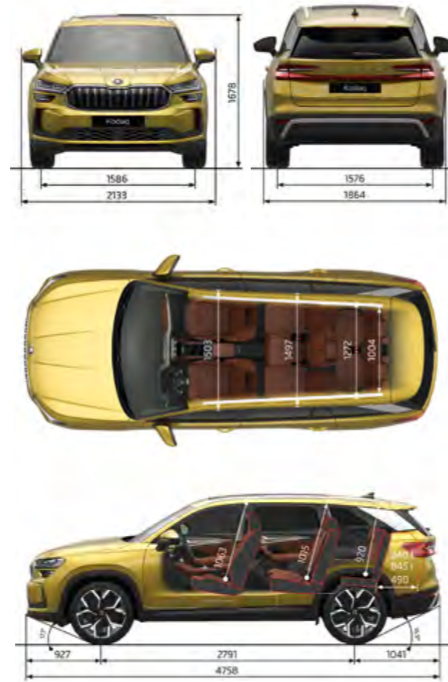
Dimensions (7-seat)
